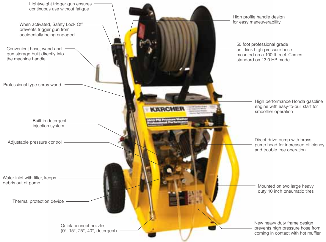
9.0 HP 3000 PSI / 13.0 HP 3600 PSI (SHOWN)
